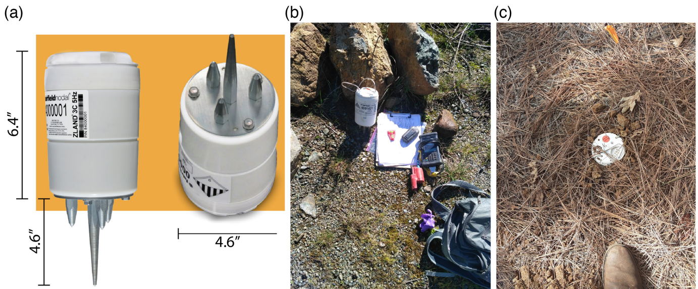
Figure 4. (a) Magseis Fairfield ZLand three-component nodal seismometer with dimensions (see Data and Resources ). (b) The ZLand seismometer is readily deployed with a handheld deployment tool and terminal after preliminary experiment geometry is created using Magseis Fairfield's proprietary software. Compass (not shown) and bubble level are used to properly orient the instrument. Redundant Global Positioning System (GPS) locations were taken with a handheld GPS. (c) Typical example of an installation prior to complete burial (shoe for scale). Locations were marked with orange utility flags placed \sim 1 ft away from the instrument. The color version of this figure is available only in the electronic edition.
